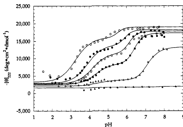
FIGURE 1: pH-induced unfolding transitions of apoMb in urea at 0 °C and 2 mM sodium citrate. Data are from experiment 1 (see text and Table I). Titrations were carried out in 0 (○), 1.0 (●), 1.5 (□), 2.0 (■), 3.0 (△), and 4.5 M urea (▲). Curves result from evaluation of the three-state stability equation (eq 15) at the urea concentrations listed above and using best-fitting parameters listed in Table II, experiment 1.
